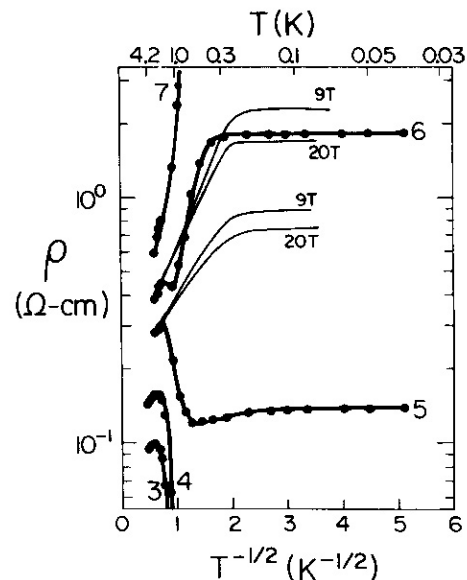
FIG. 2. Logarithm of resistivity vs T^{-1/2} for samples 3, 4, 5, 6, and 7 of Fig. 1 selected for measurement in the dilution refrigerator. Curves labeled 9 T and 20 T: measurements done in fields at that value. Unlabeled curves: zero magnetic field.
