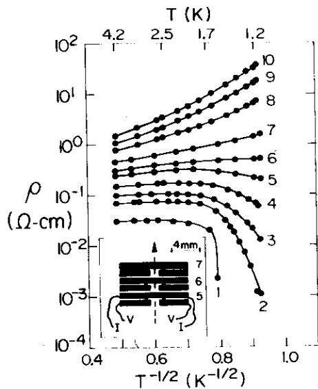
FIG. 1. Logarithm of resistivity vs T^{-1/2} between 1.2 and 4.2 K for a range of granular aluminum samples near the metal-insulator transition. The room-temperature resistivities of samples No. 1-10 are, respectively, 9.1, 13, 16, 20, 25, 28, 34, 37, 40, and 41 mΩ cm. Inset: Relative positions of samples 5, 6, and 7 in the evaporator. The other samples were coplanar and in sequence along the dashed line.
