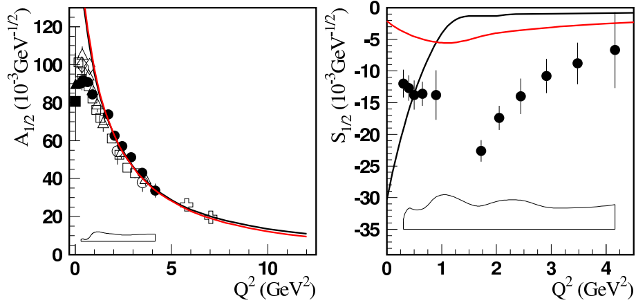
FIG. 51. The \gamma^*p \rightarrow N(1535)S_{11} transition amplitudes. The amplitudes extracted from the CLAS and JLab/Hall C data on ep \rightarrow enp are: the stars [55], the open boxes [9], the open circles [56], the crosses [57], and the rhombuses [19, 40]. c_{N^*}^{(1)} = 0.88 \pm 0.03 , c_{N^*}^{(2)} = 0.94 \pm 0.03 . Other legend is as for Fig. 48.
