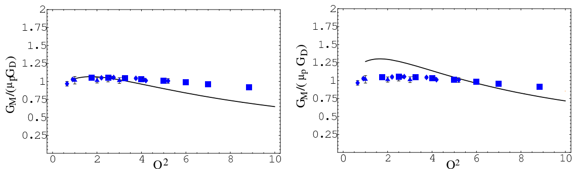
FIG. 37. LCSR results for the magnetic proton form factor (normalized to the dipole formula) for a realistic model of nucleon distribution amplitudes [202]. Left panel: Leading order (LO); right panel: next-to-leading order (NLO) for twist-three contributions. Figure adapted from Ref. [203].
