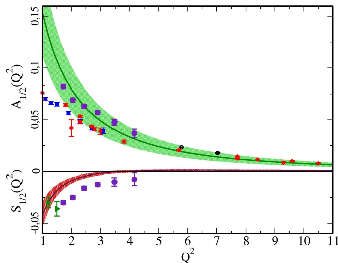
FIG. 36. The LCSR calculation for the helicity amplitudes A_{1/2}(Q^2) and S_{1/2}(Q^2) for the electroproduction of the N^*(1535) resonance using the lattice results for the lowest moments of the N^*(1535) DAs. The curves are obtained using the central values of the lattice parameters, and the shaded areas show the corresponding uncertainty. Figure taken from Ref. [179].
