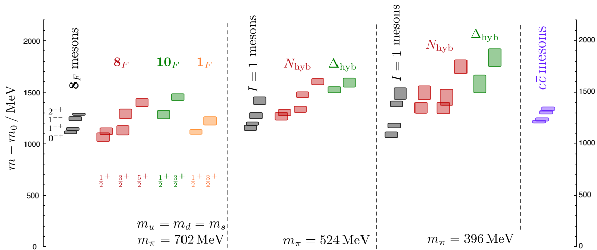
FIG. 23. Results from Ref. [14, 89, 90] showing the spectrum of hybrid mesons and baryons for three light quark masses. Mass scale is m - m_\rho for light quark mesons, m - m_{J/\Psi} , and m - m_N for baryons to approximately subtract the effect of differing numbers of quarks.
