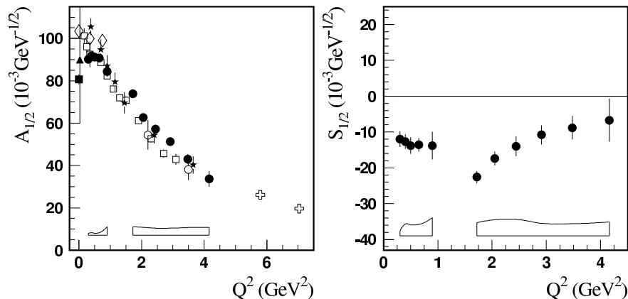
FIG. 15. Transverse electrocoupling A_{1/2} of the \gamma^*p \rightarrow S_{11}(1535) transition. The full circles are the electrocouplings extracted from N\pi electroproduction data [19]. The electrocouplings extracted from N\eta electroproduction data are: the stars [55], the open boxes [9], the open circles [56], the crosses [57], and the rhombuses [39, 40]. The full box and triangle at Q^2 = 0 correspond to [4] and the CLAS N\pi [26] photoproduction results, respectively.
